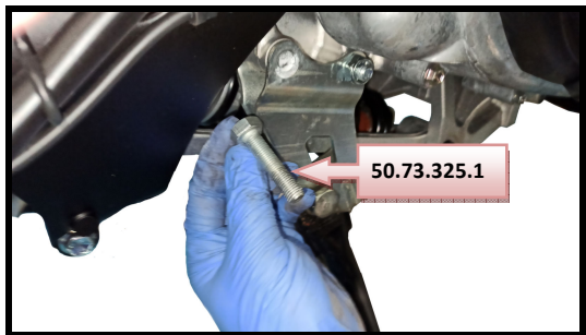
Inserire la vite corta 50.73.325.1. Insert the short screw 50.73.325.1
